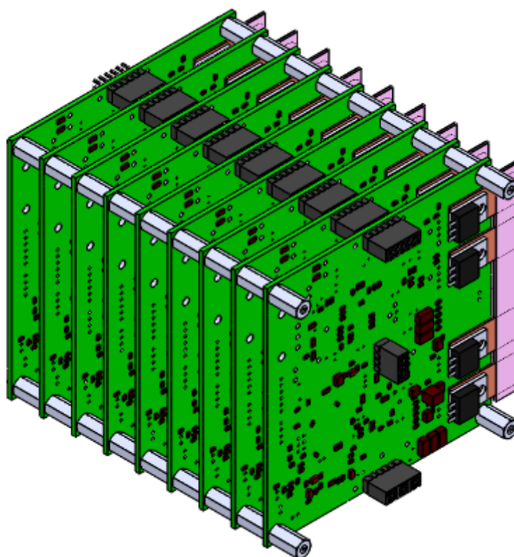
Fig. 1: ICE daughter modules stacked together.
