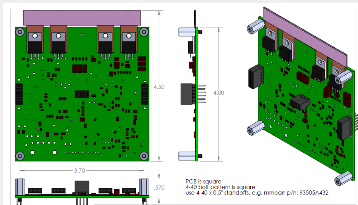
PCB dimensions.
