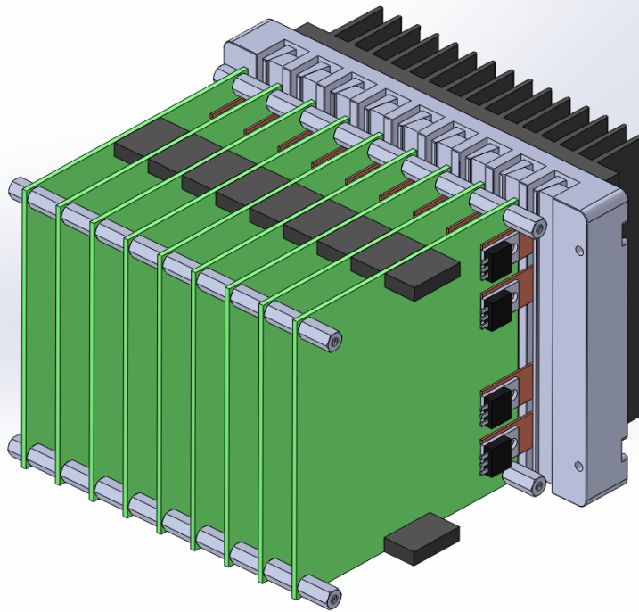
Overall pcb heatsink stackup
