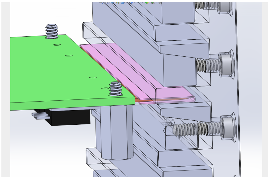
Detail view of wedge clamp. Pink material is Sil-Pad for electrical isolation.
